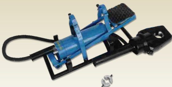
HEXPRESS HYF - 400 (Hydraulic Foot Operated) Crimping Capacity : 50mm 2 to 400mm 2 Weight : 17kgs
